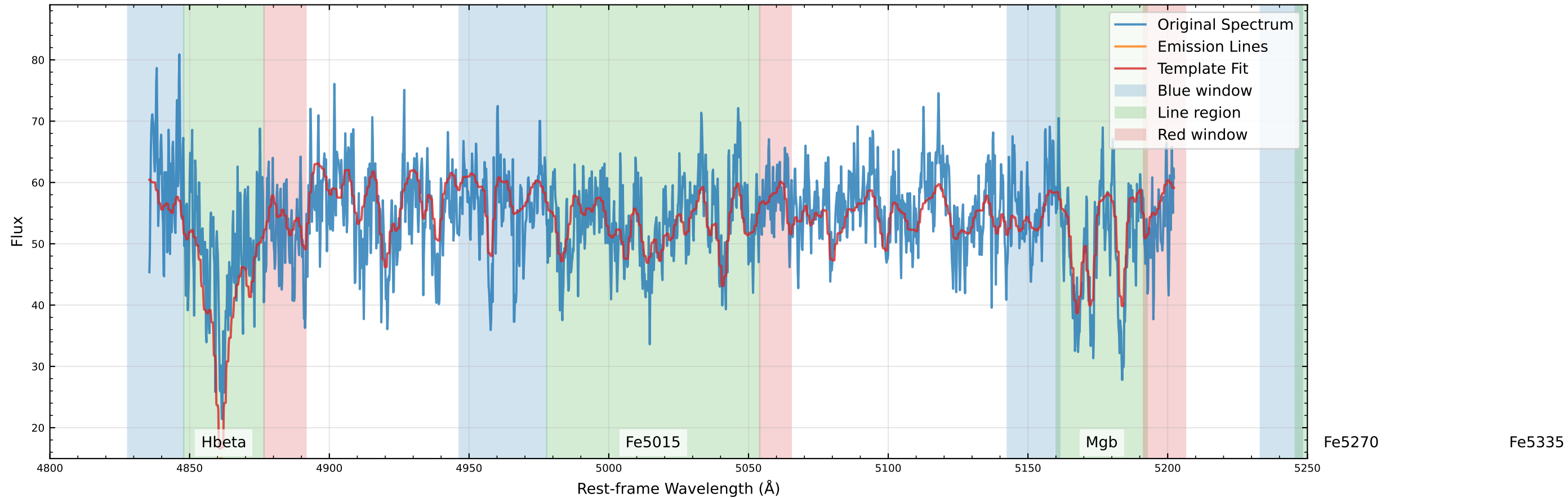
Original Data Comparison (v_star=9.9 km/s, v_gas=-0.3 km/s)
