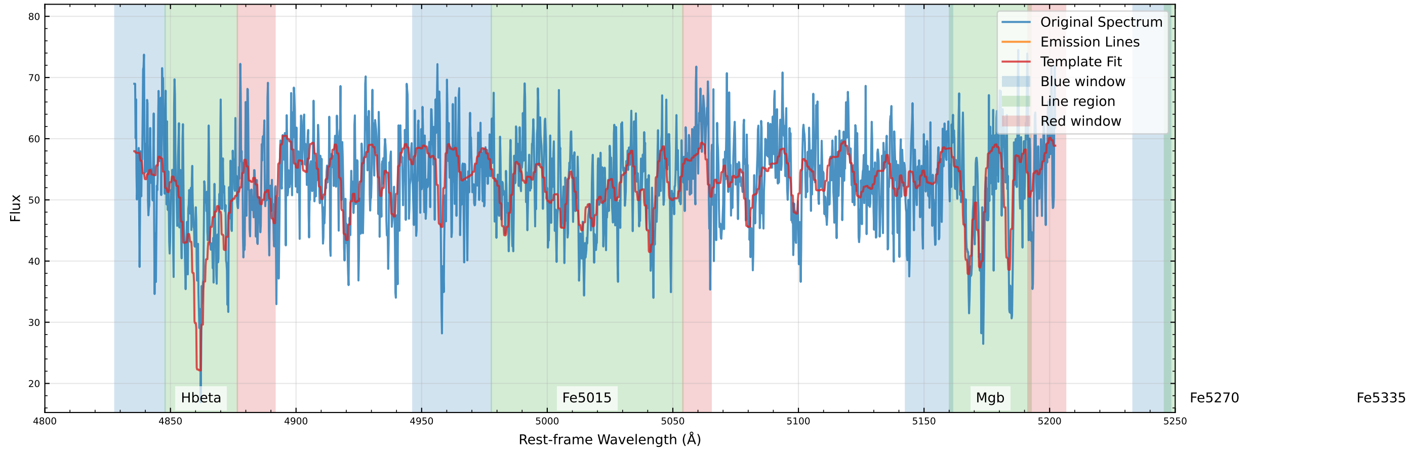
Original Data Comparison (v_star=48.3 km/s, v_gas=64.4 km/s)
