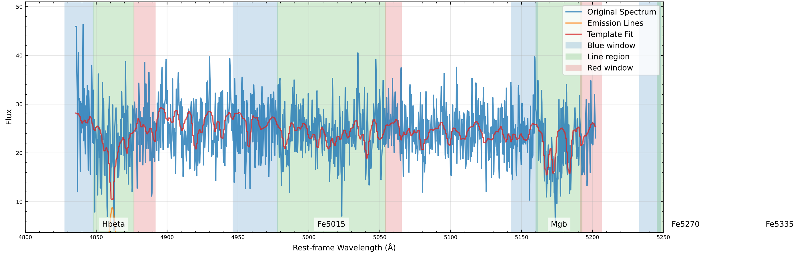
Original Data Comparison (v_star=80.9 km/s, v_gas=75.5 km/s)
