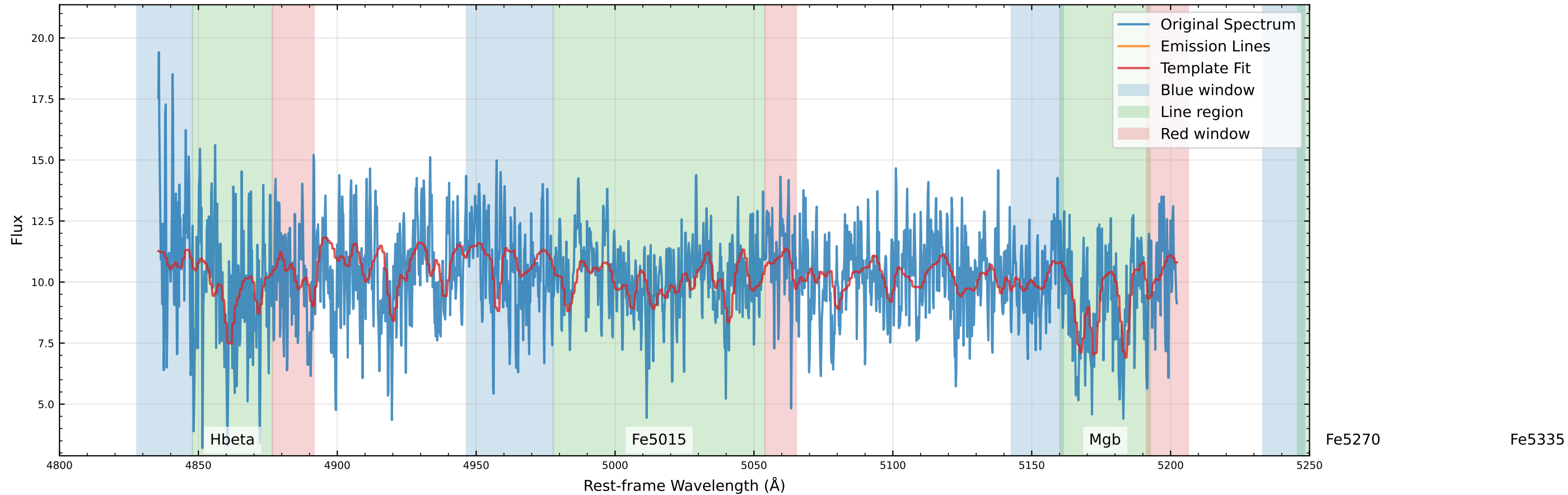
Original Data Comparison (v_star=-81.8 km/s, v_gas=-109.8 km/s)
