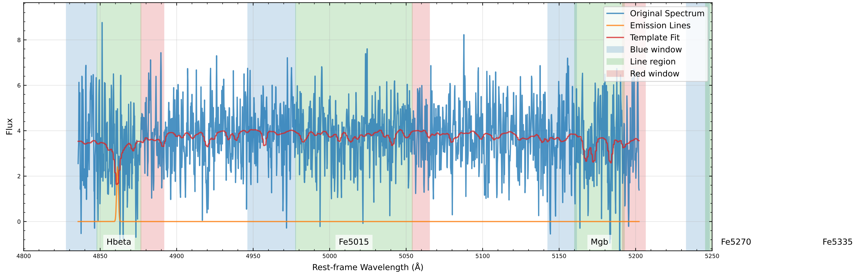
Original Data Comparison (v_star=-7.7 km/s, v_gas=-27.5 km/s)
