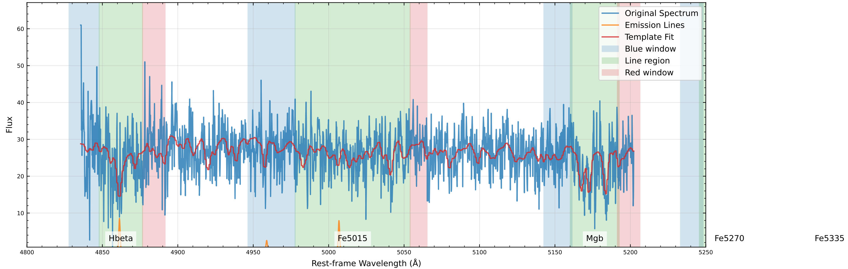
Original Data Comparison (v_star=44.7 km/s, v_gas=22.9 km/s)
