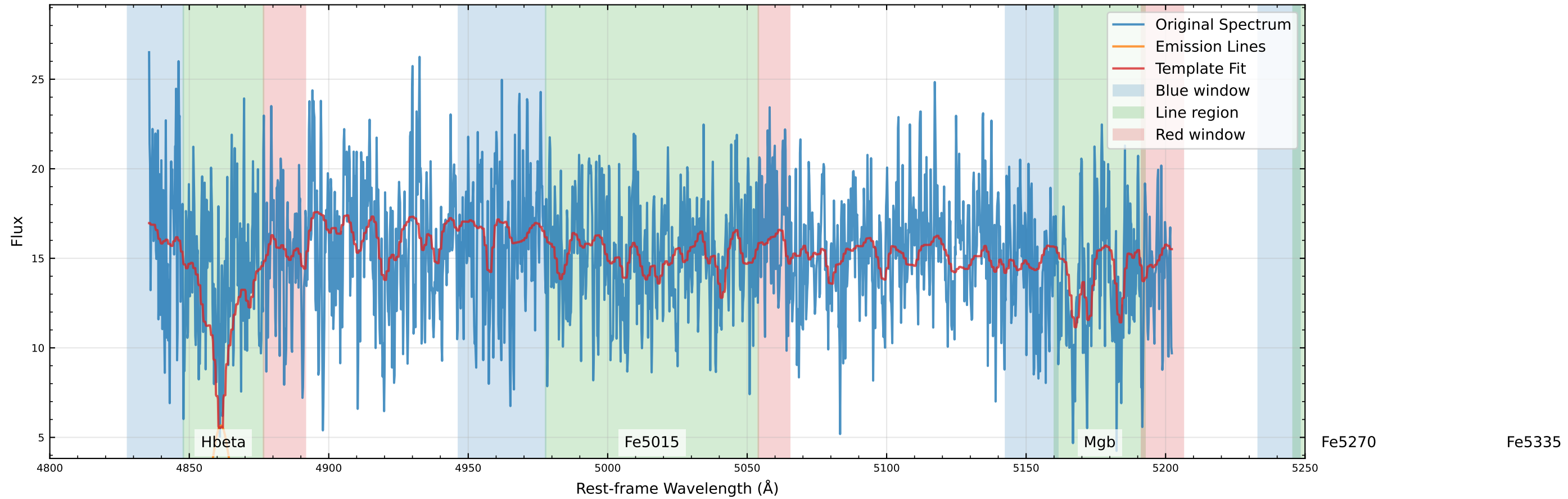
Original Data Comparison (v_star=-24.2 km/s, v_gas=-70.9 km/s)
