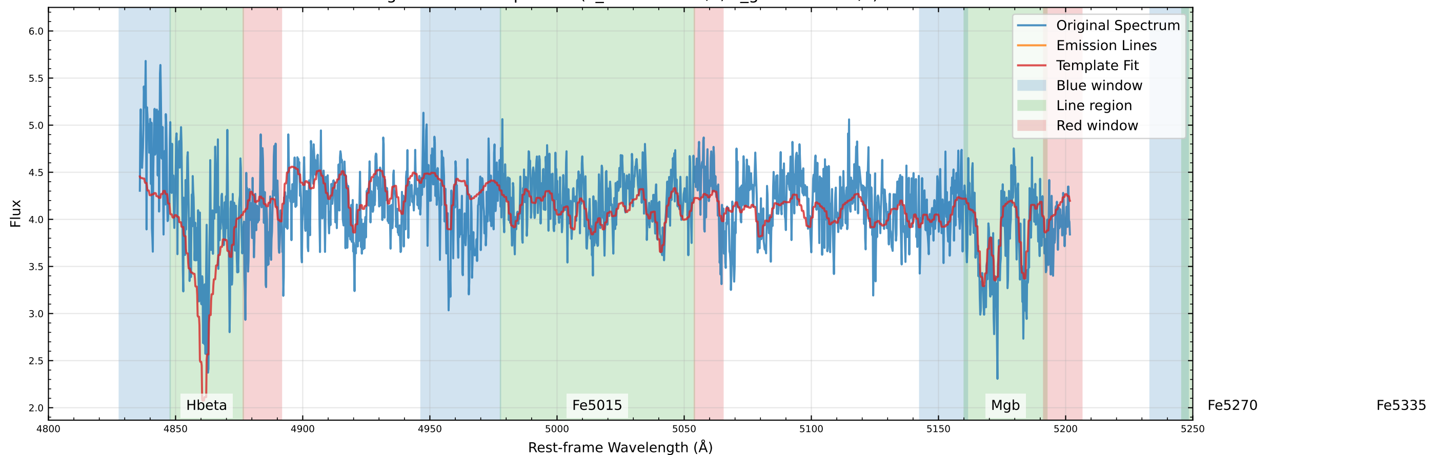
Original Data Comparison (v_star=7.5 km/s, v_gas=14.4 km/s)
