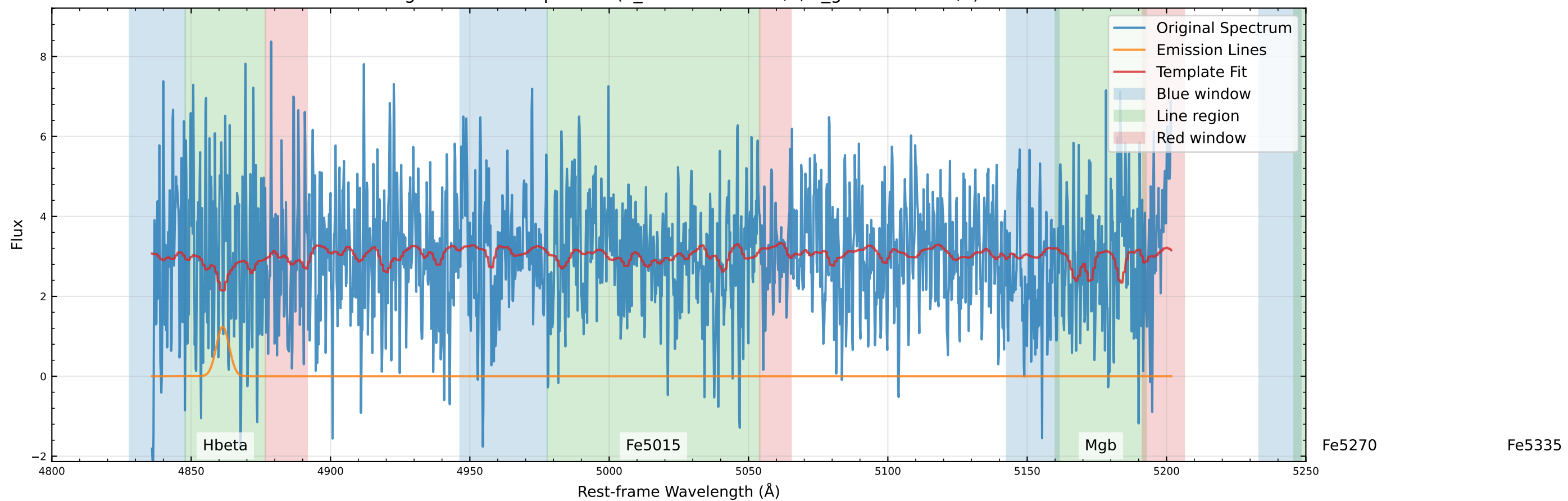
Original Data Comparison (v_star=-170.6 km/s, v_gas=-84.0 km/s)
