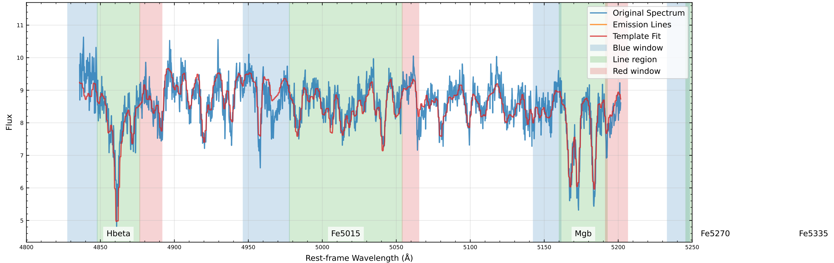
Original Data Comparison (v_star=2.8 km/s, v_gas=94.8 km/s)
