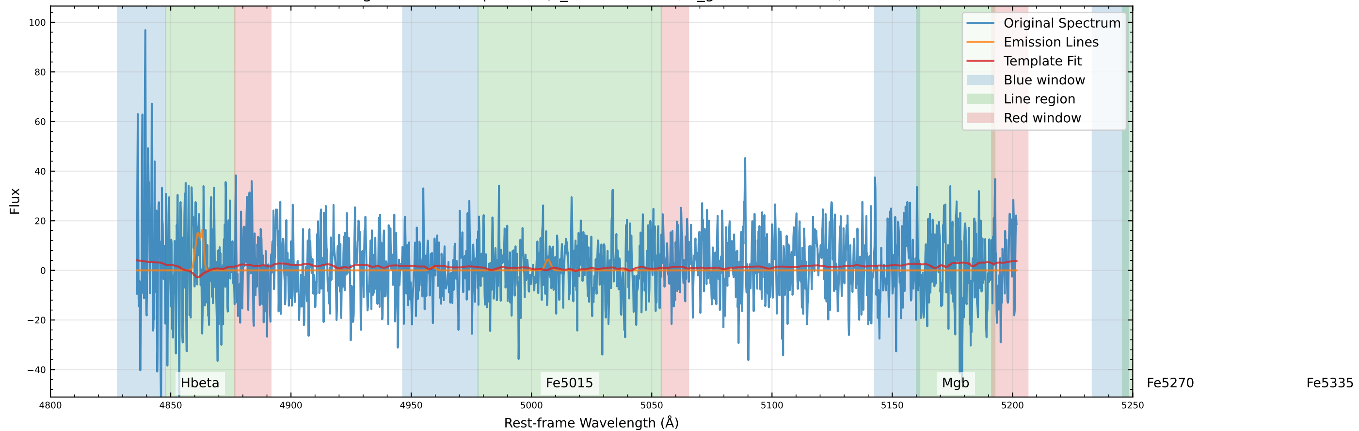
Original Data Comparison (v_star=0.0 km/s, v_gas=-108.0 km/s)
