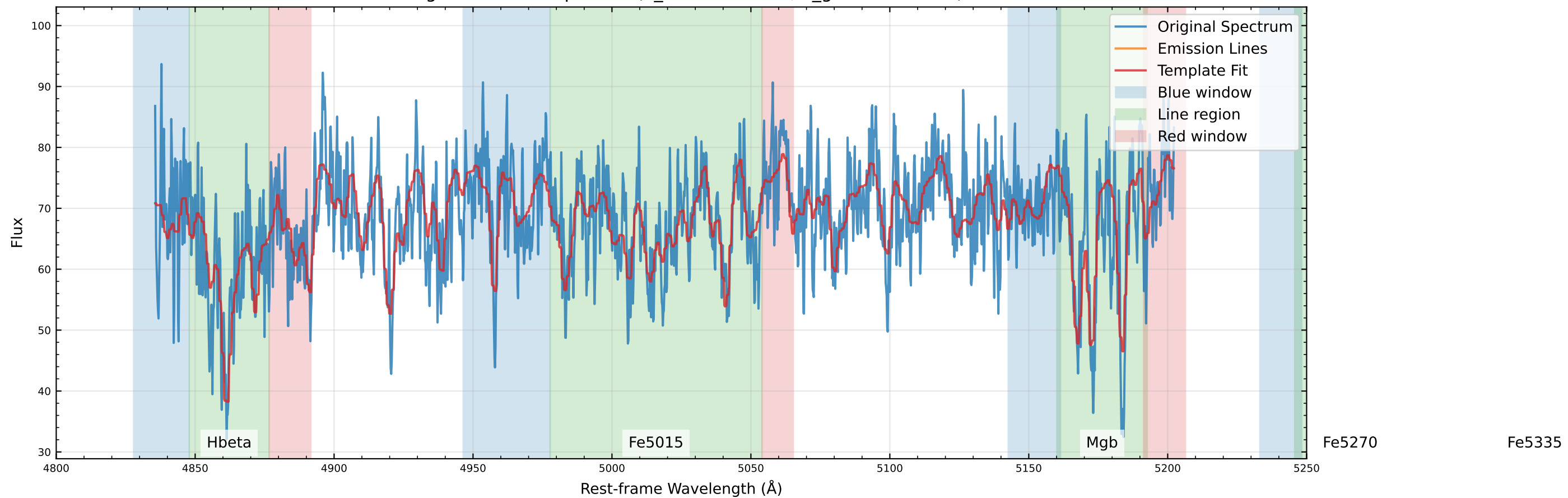
Original Data Comparison (v_star=8.8 km/s, v_gas=81.1 km/s)
