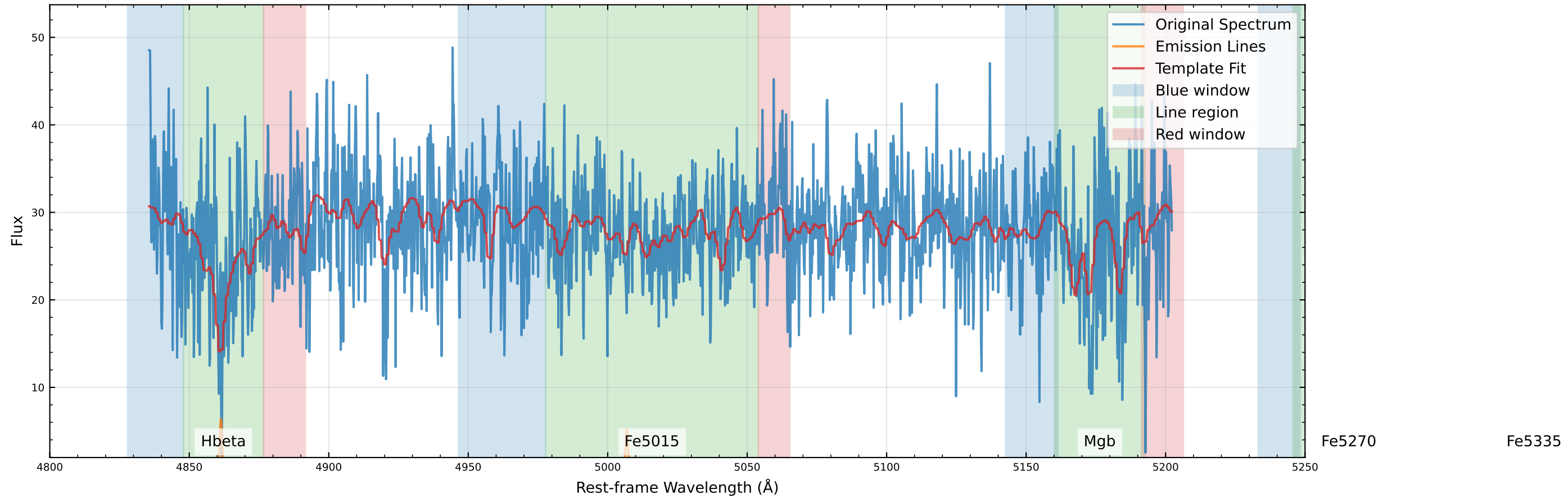
Original Data Comparison (v_star=45.1 km/s, v_gas=92.3 km/s)
