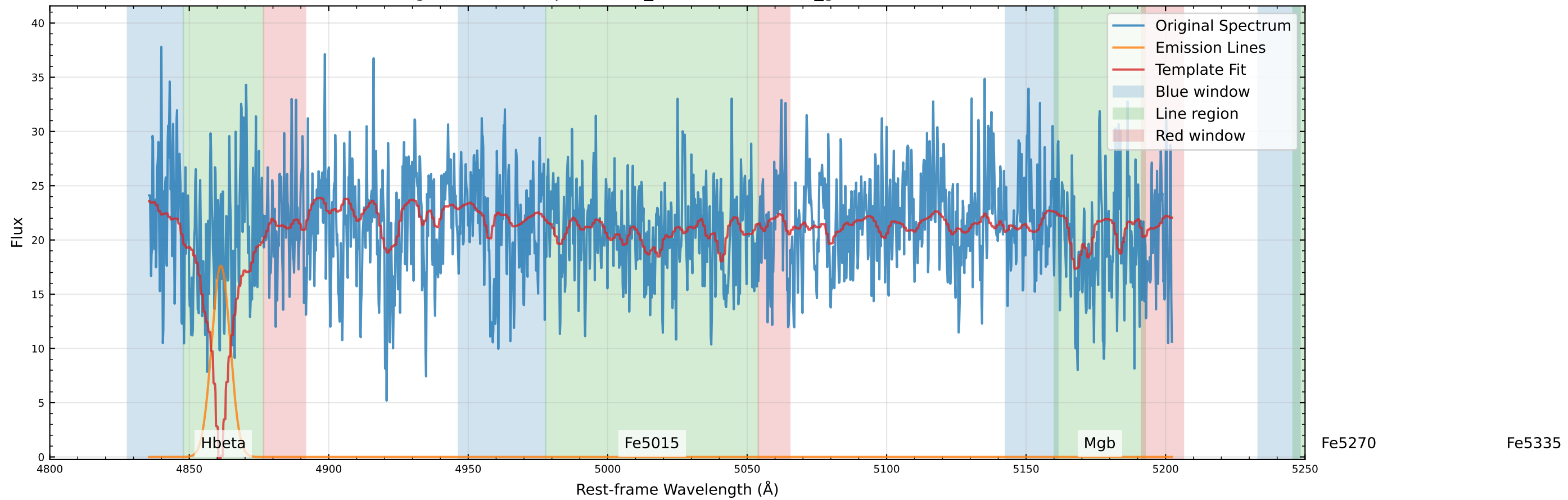
Original Data Comparison (v_star=51.3 km/s, v_gas=58.8 km/s)
