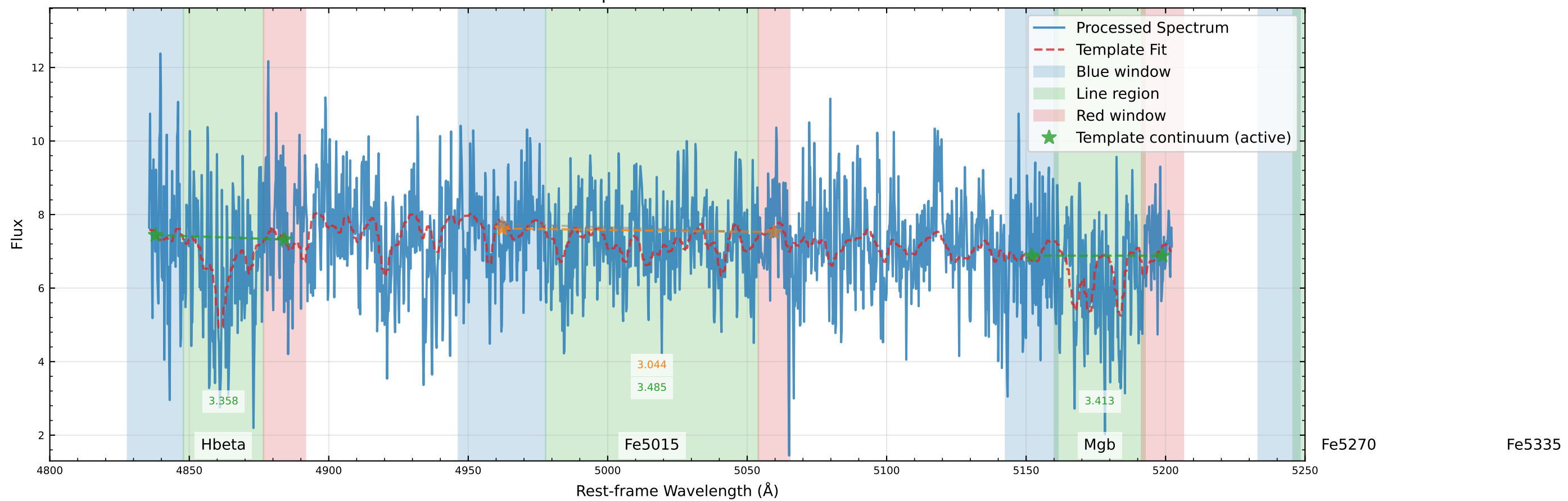
Processed Spectrum with Continuum Fits
