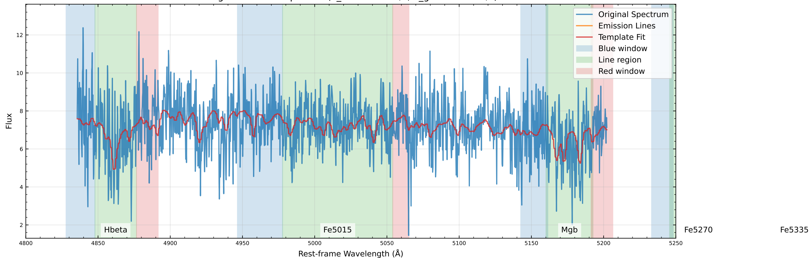
Original Data Comparison (v_star=5.6 km/s, v_gas=62.0 km/s)
