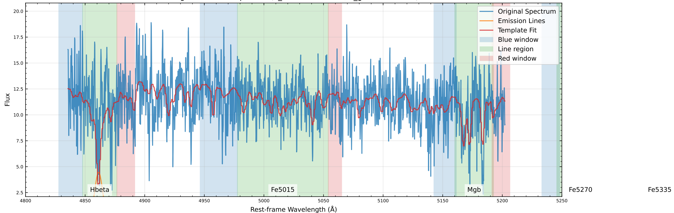
Original Data Comparison (v_star=-12.9 km/s, v_gas=26.5 km/s)
