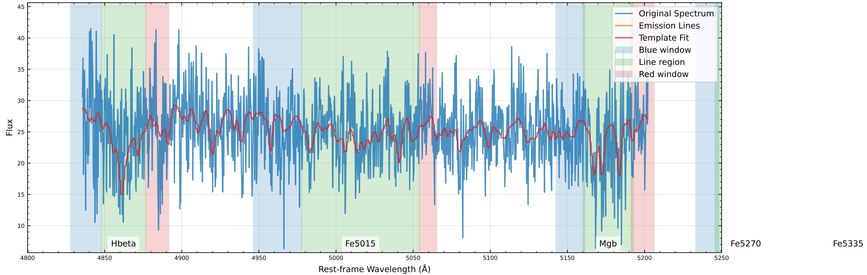
Original Data Comparison (v_star=-2.3 km/s, v_gas=49.7 km/s)
