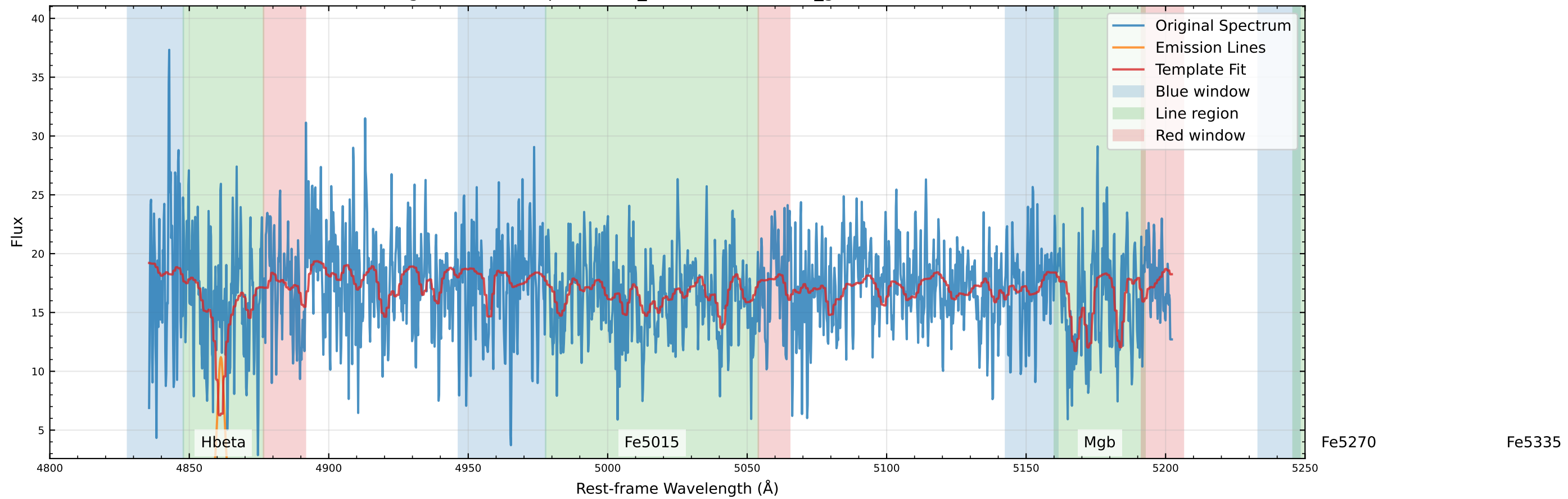
Original Data Comparison (v_star=-63.8 km/s, v_gas=-54.0 km/s)
