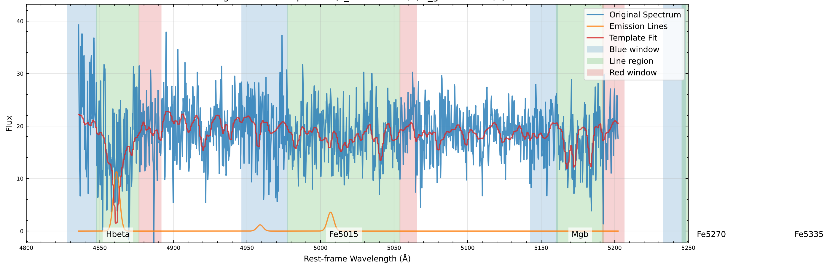
Original Data Comparison (v_star=9.2 km/s, v_gas=-4.6 km/s)
