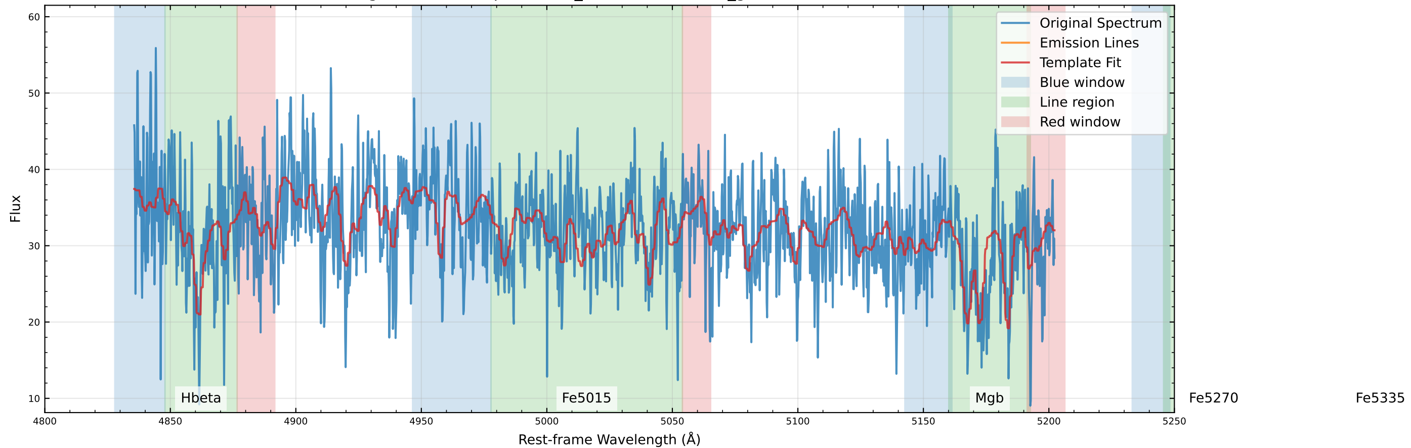
Original Data Comparison (v_star=15.8 km/s, v_gas=103.4 km/s)
