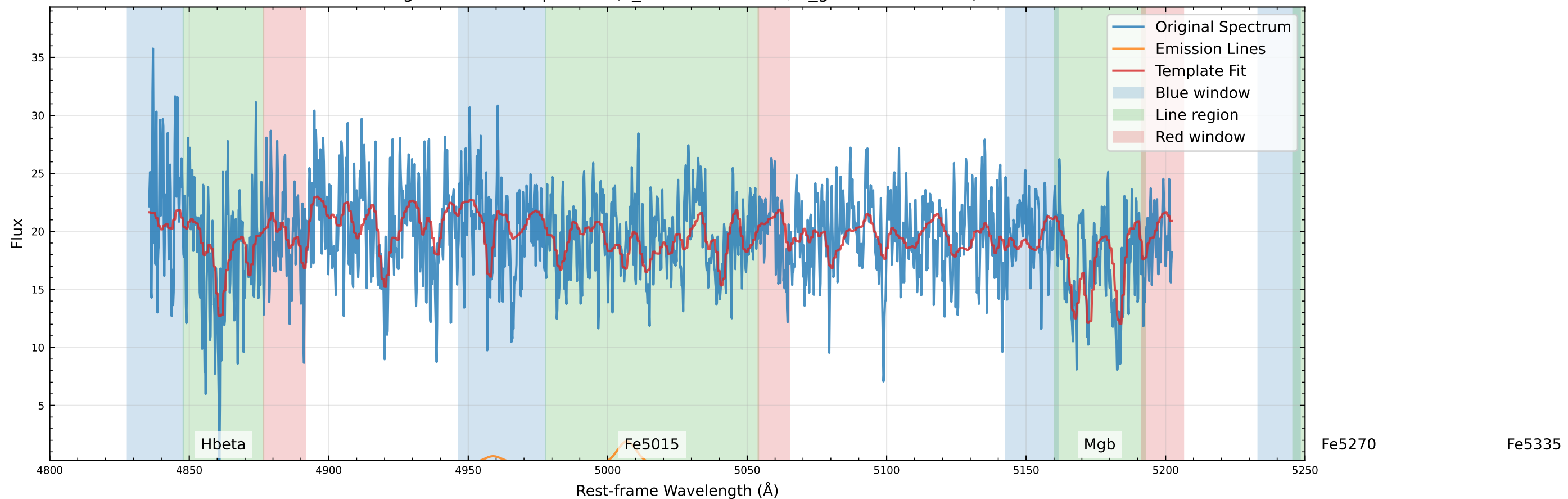
Original Data Comparison (v_star=-37.7 km/s, v_gas=-164.7 km/s)
