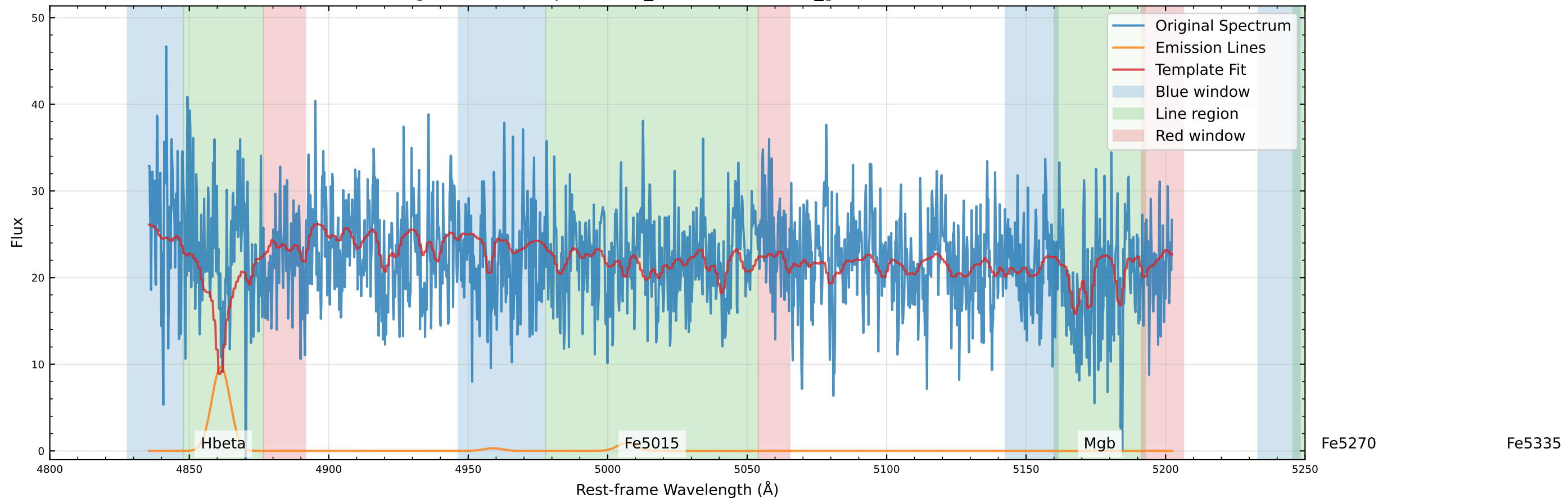
Original Data Comparison (v_star=26.1 km/s, v_gas=66.4 km/s)
