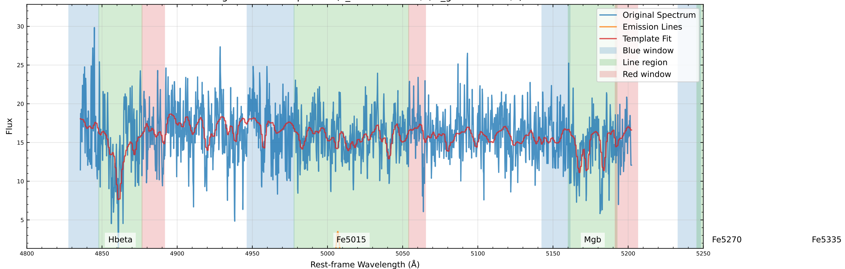
Original Data Comparison (v_star=-53.4 km/s, v_gas=39.5 km/s)
