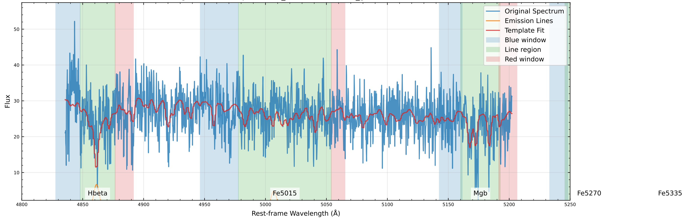
Original Data Comparison (v_star=22.4 km/s, v_gas=58.4 km/s)
