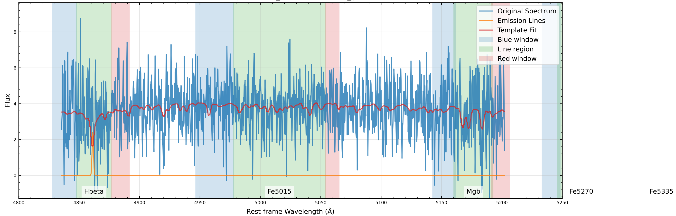
Original Data Comparison (v_star=-7.7 km/s, v_gas=-27.5 km/s)
