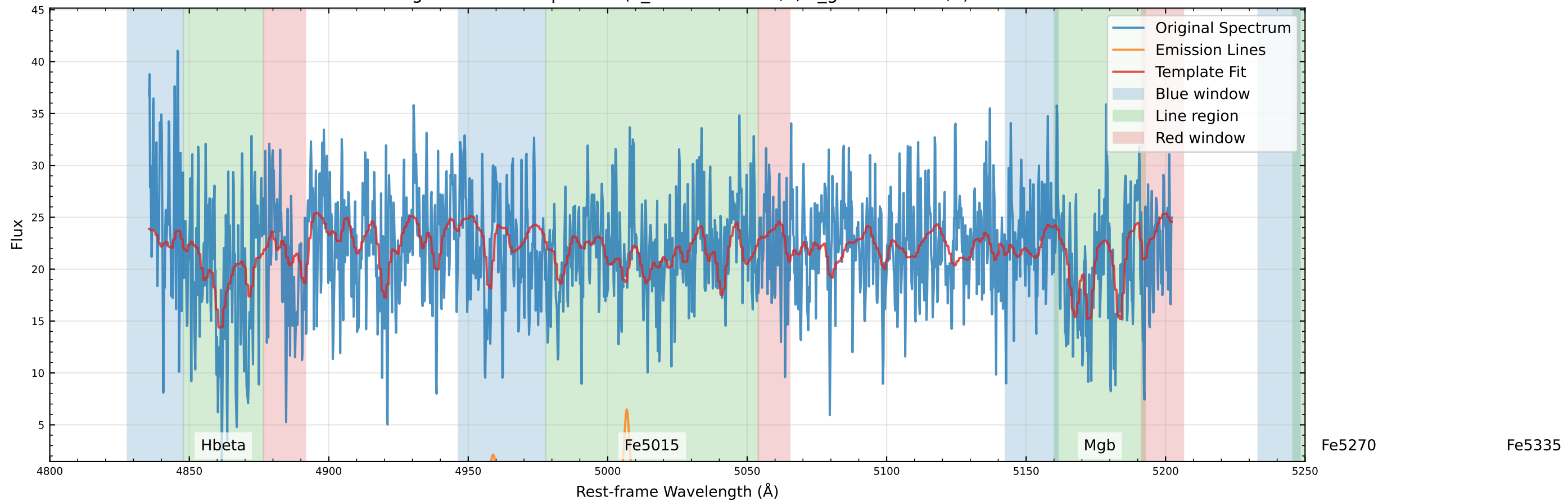
Original Data Comparison (v_star=-29.0 km/s, v_gas=94.2 km/s)
