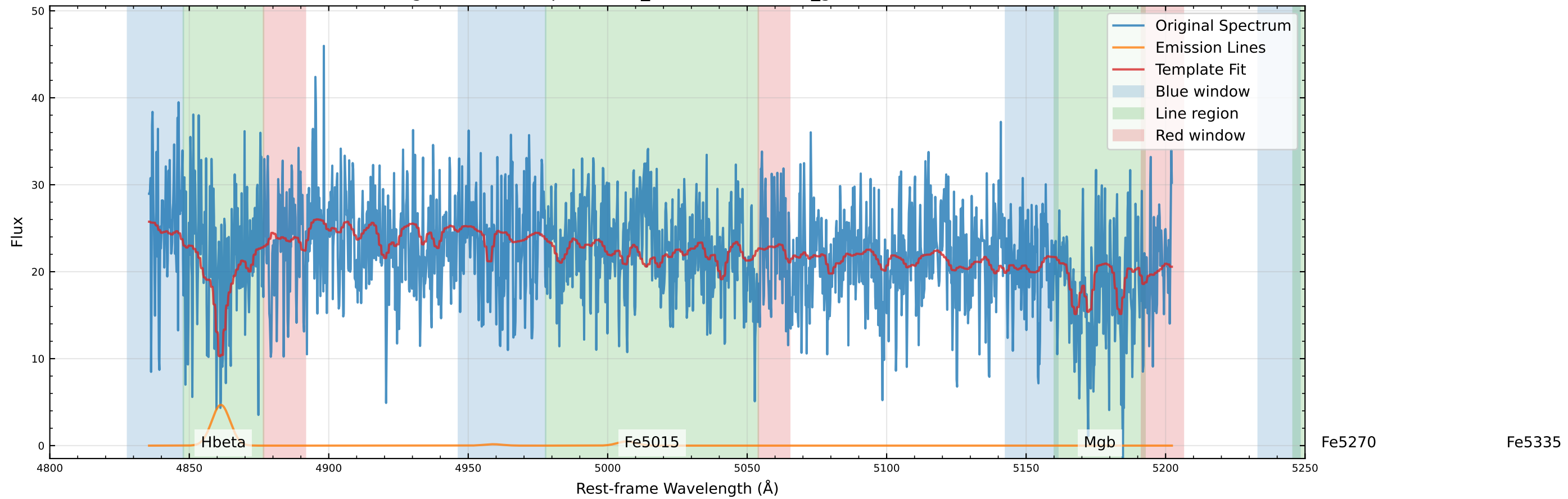
Original Data Comparison (v_star=15.5 km/s, v_gas=-27.3 km/s)
