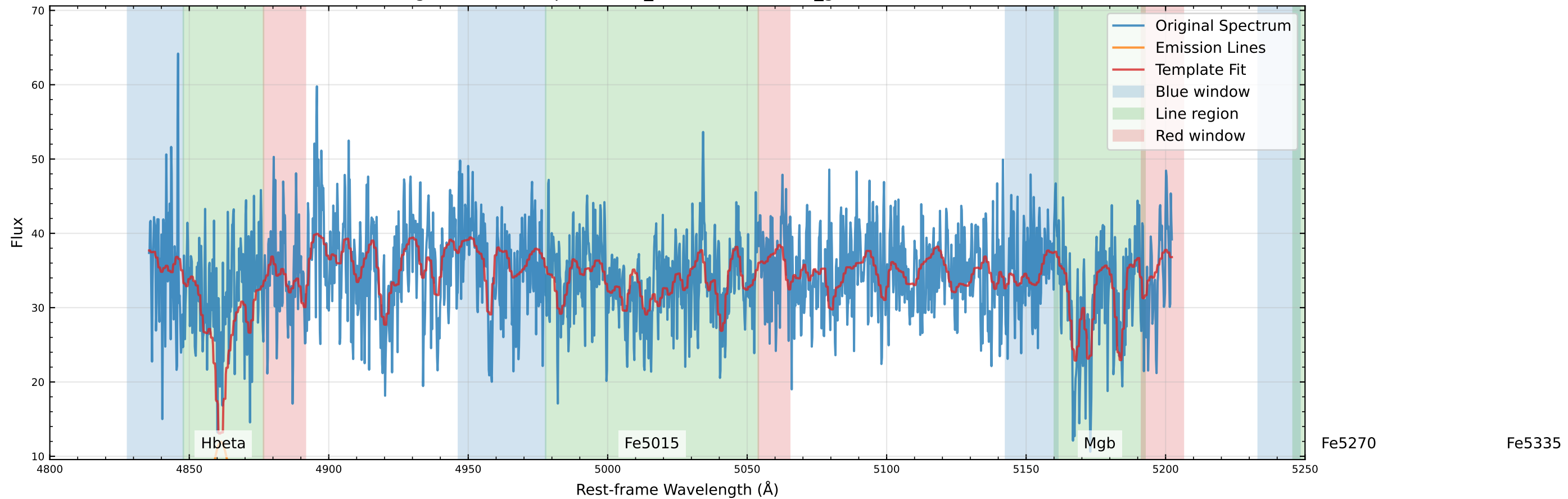
Original Data Comparison (v_star=23.6 km/s, v_gas=92.2 km/s)
