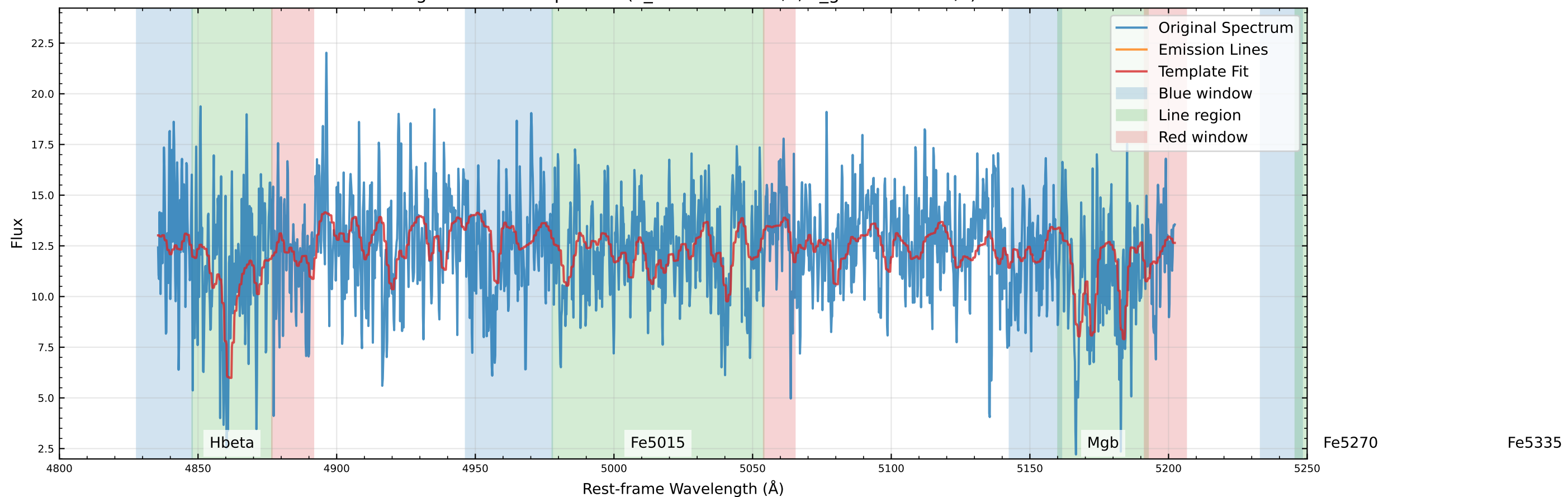
Original Data Comparison (v_star=-63.3 km/s, v_gas=-24.8 km/s)
