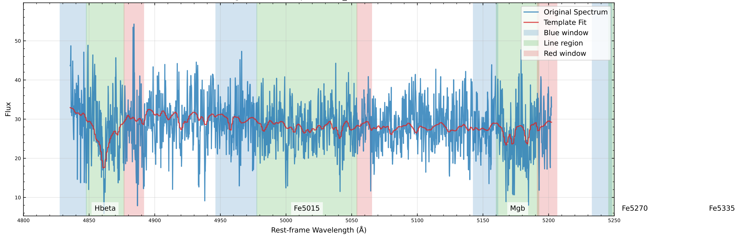
Original Data Comparison ( v_{\text{star}}=41.6 km/s)
