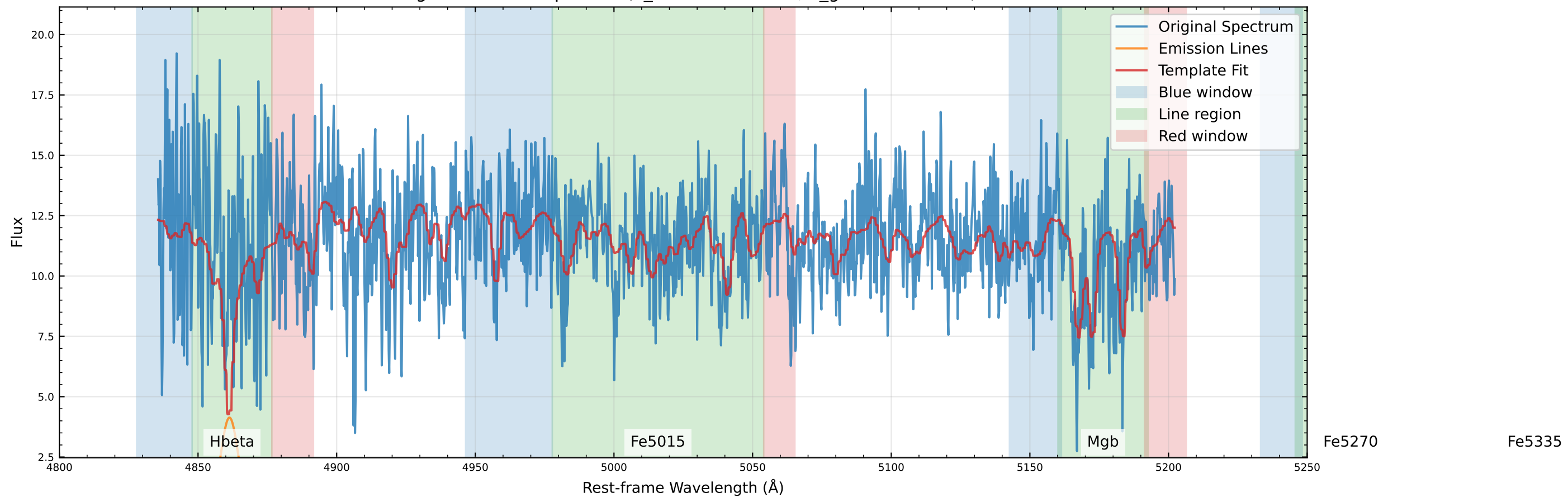
Original Data Comparison (v_star=-42.2 km/s, v_gas=-96.2 km/s)
