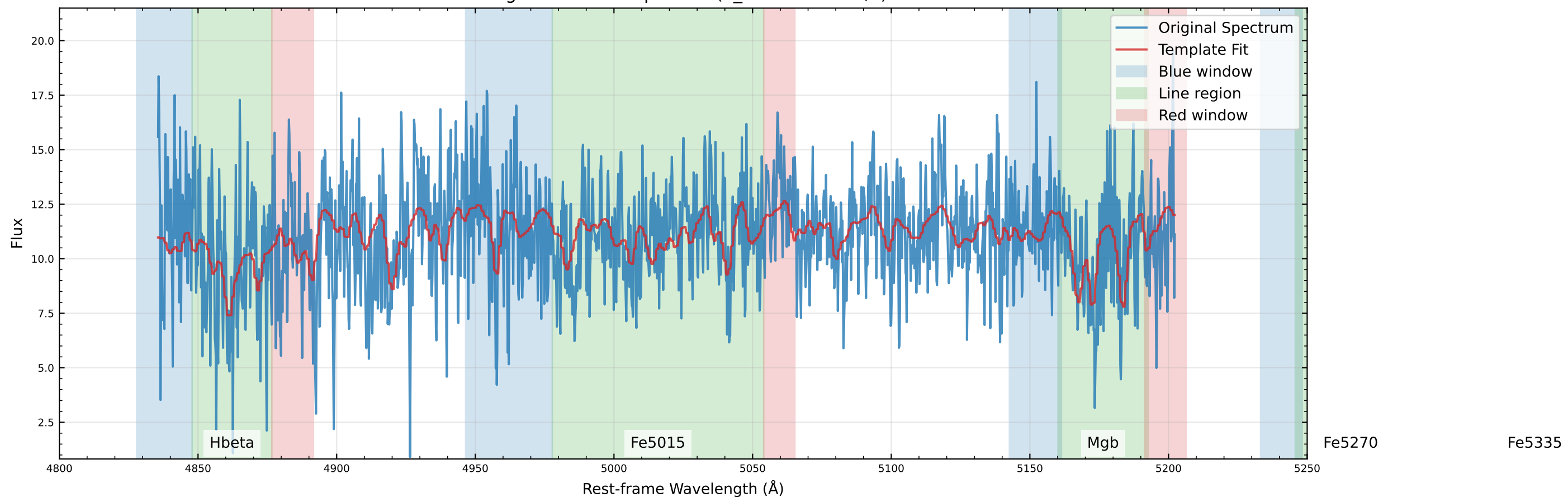
Original Data Comparison (v_star=34.1 km/s)
