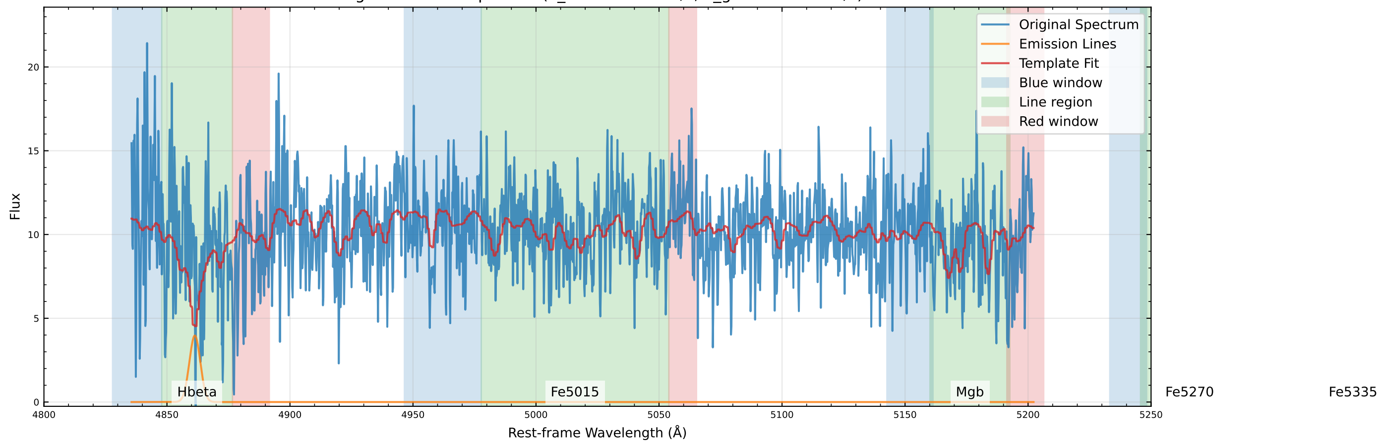
Original Data Comparison (v_star=-17.4 km/s, v_gas=-162.6 km/s)
