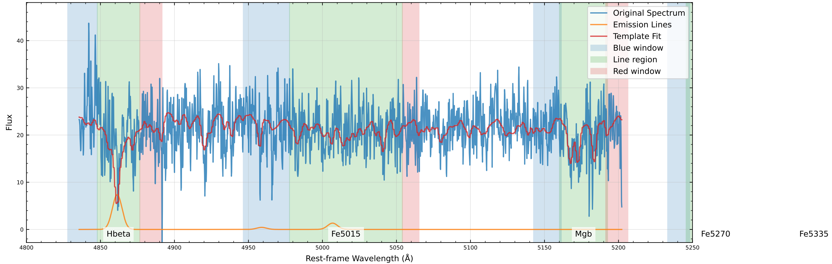
Original Data Comparison (v_star=27.1 km/s, v_gas=18.3 km/s)
