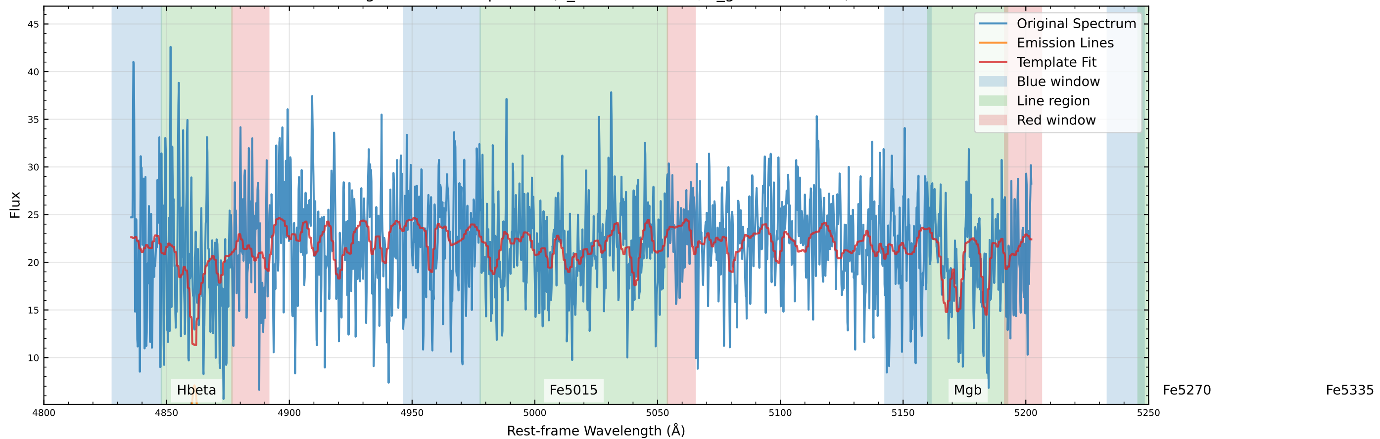
Original Data Comparison (v_star=71.6 km/s, v_gas=76.1 km/s)
