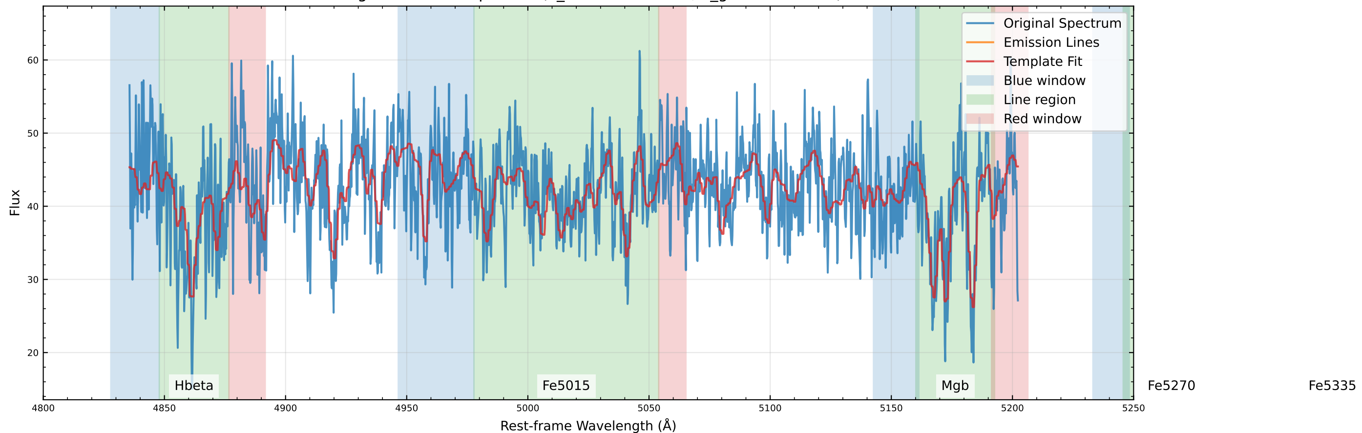
Original Data Comparison (v_star=-13.5 km/s, v_gas=10.0 km/s)
