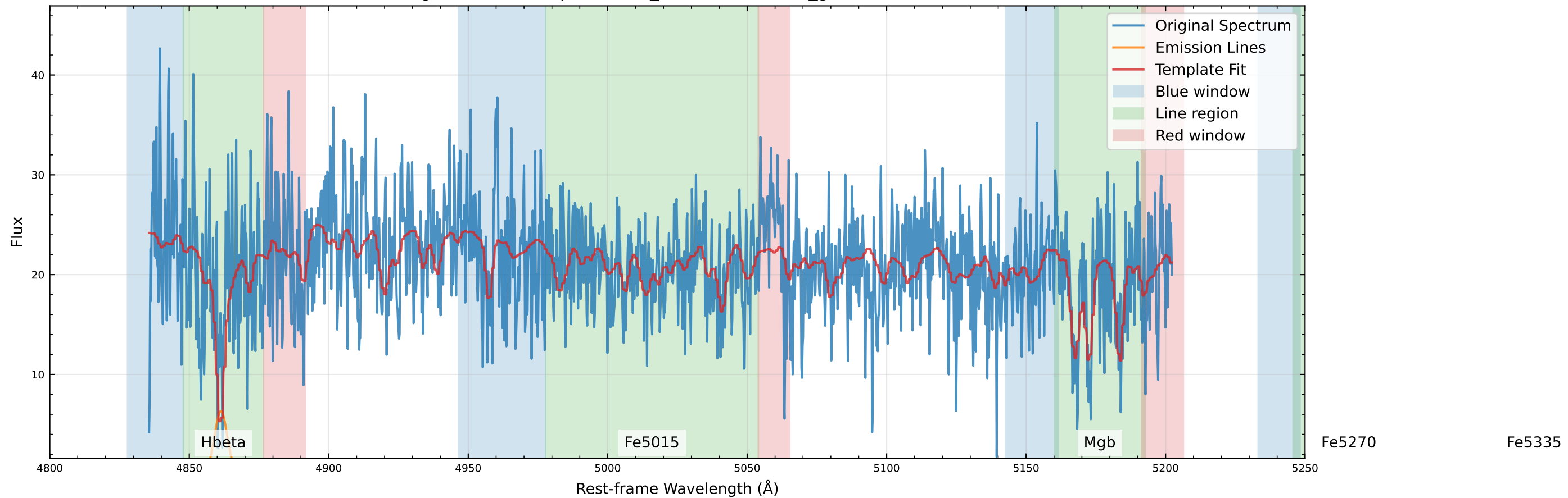
Original Data Comparison (v_star=6.6 km/s, v_gas=51.0 km/s)
