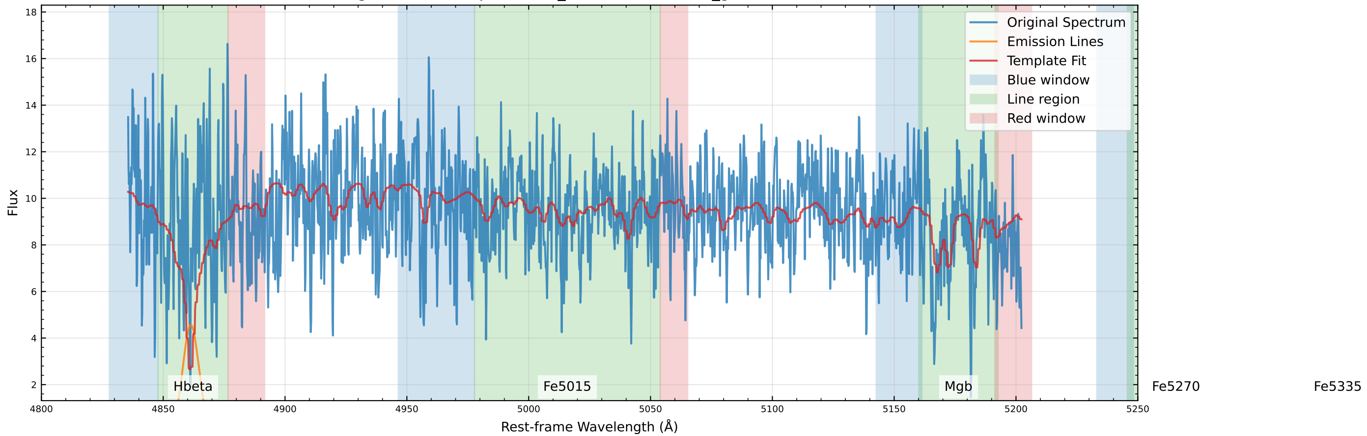
Original Data Comparison (v_star=-30.1 km/s, v_gas=31.1 km/s)
