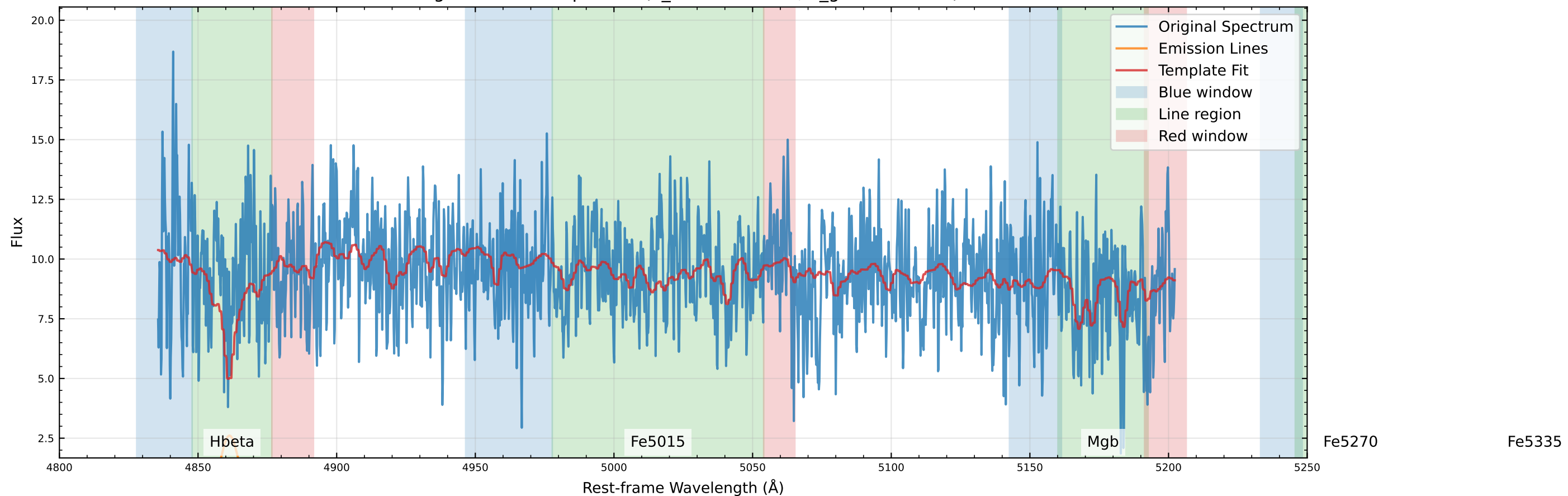
Original Data Comparison (v_star=4.4 km/s, v_gas=6.4 km/s)
