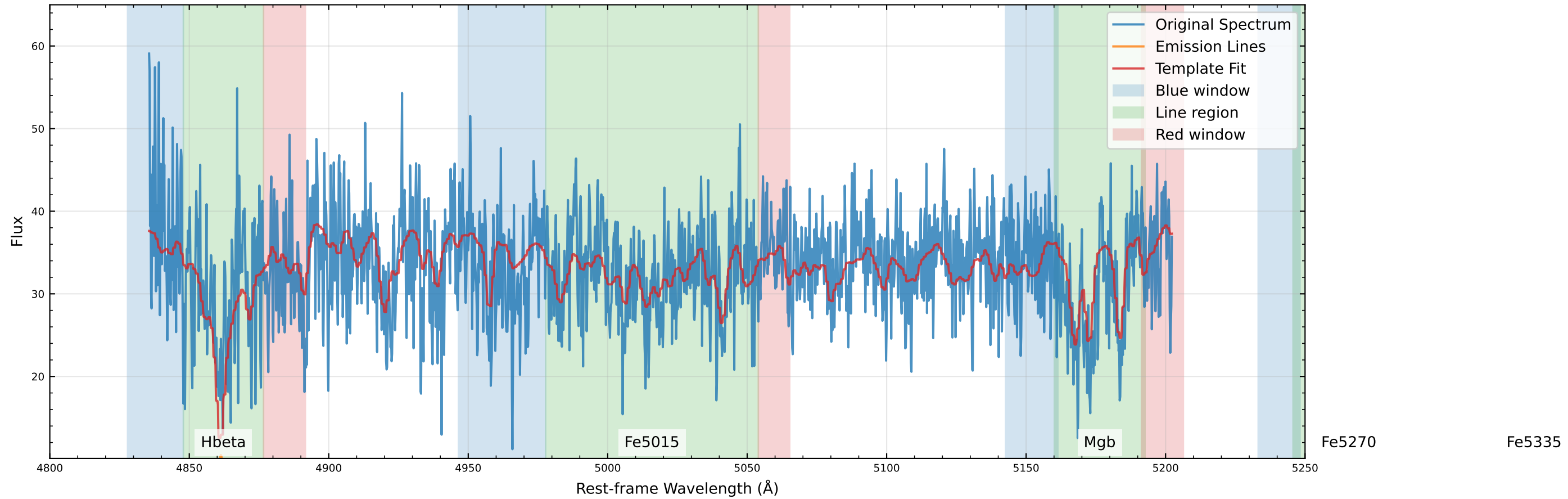
Original Data Comparison (v_star=18.9 km/s, v_gas=47.7 km/s)
