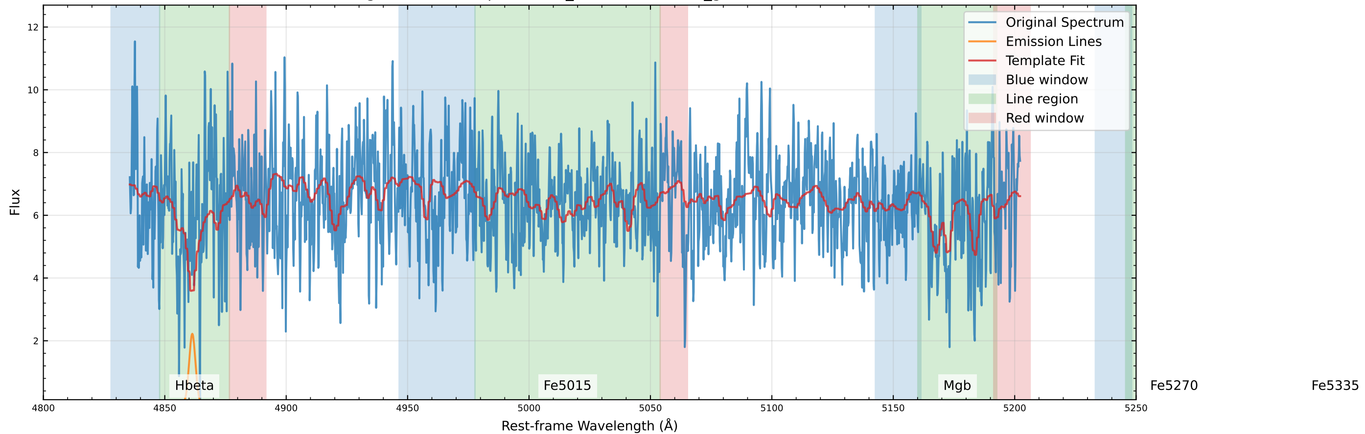
Original Data Comparison (v_star=0.5 km/s, v_gas=24.4 km/s)
