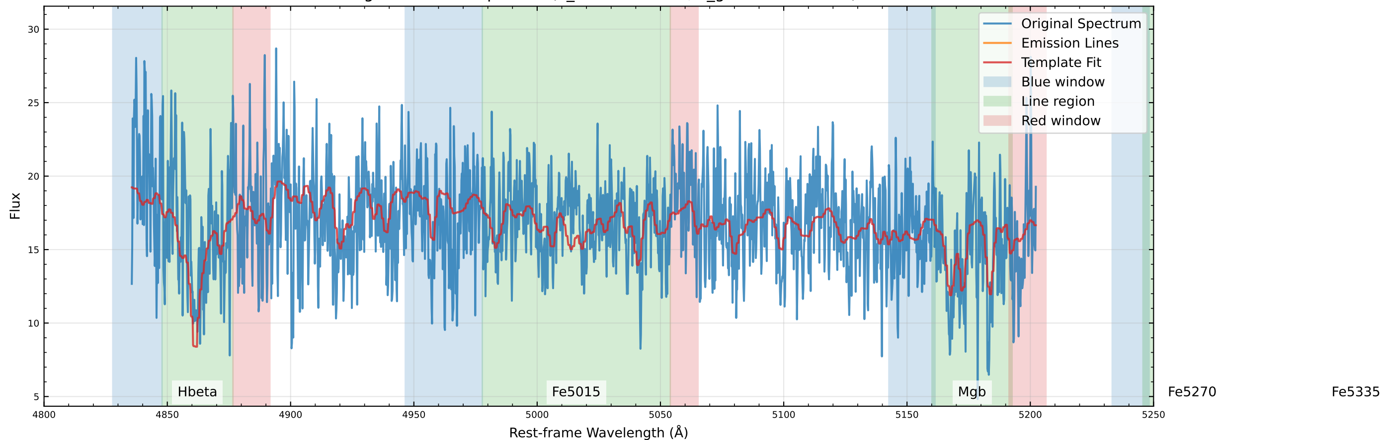
Original Data Comparison (v_star=7.9 km/s, v_gas=-196.2 km/s)
