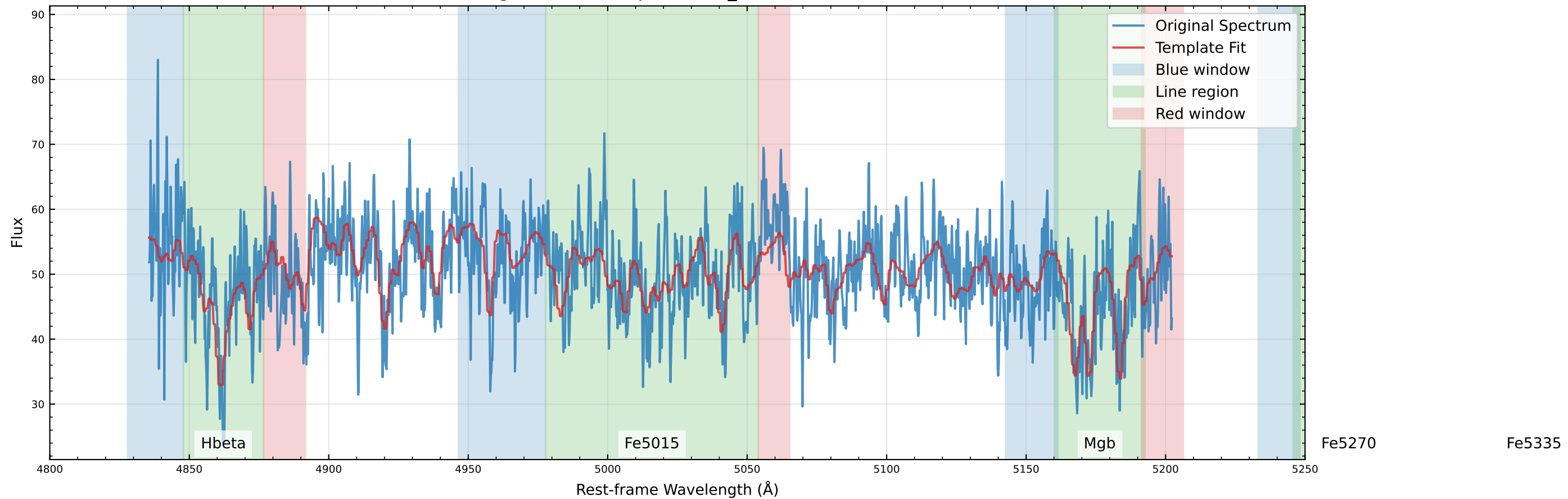
Original Data Comparison (v_star=33.4 km/s)
