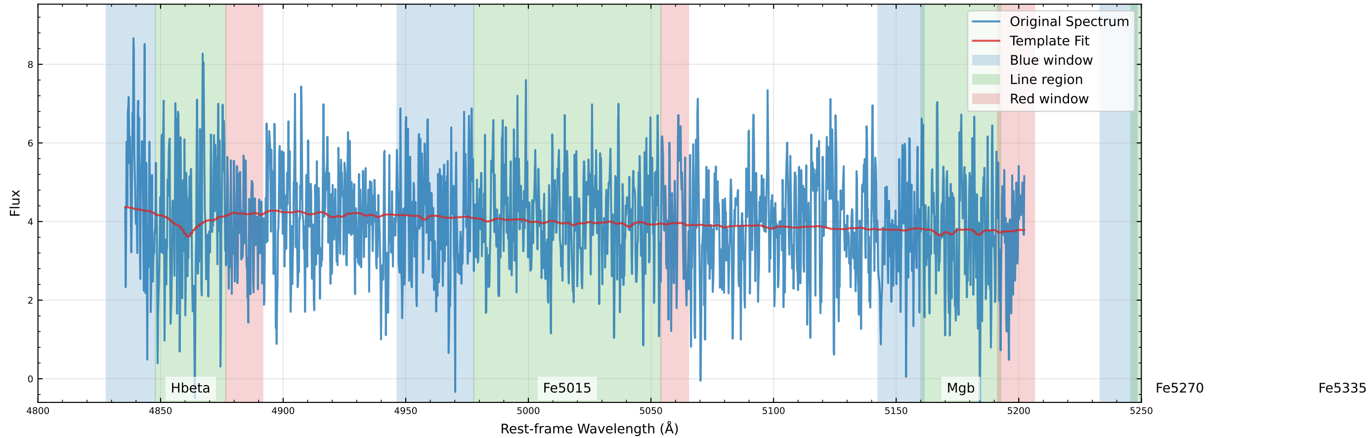
Original Data Comparison (v_star=87.6 km/s)
