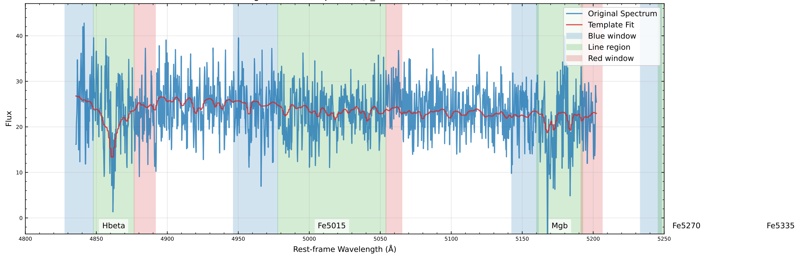
Original Data Comparison (v_star=27.0 km/s)
