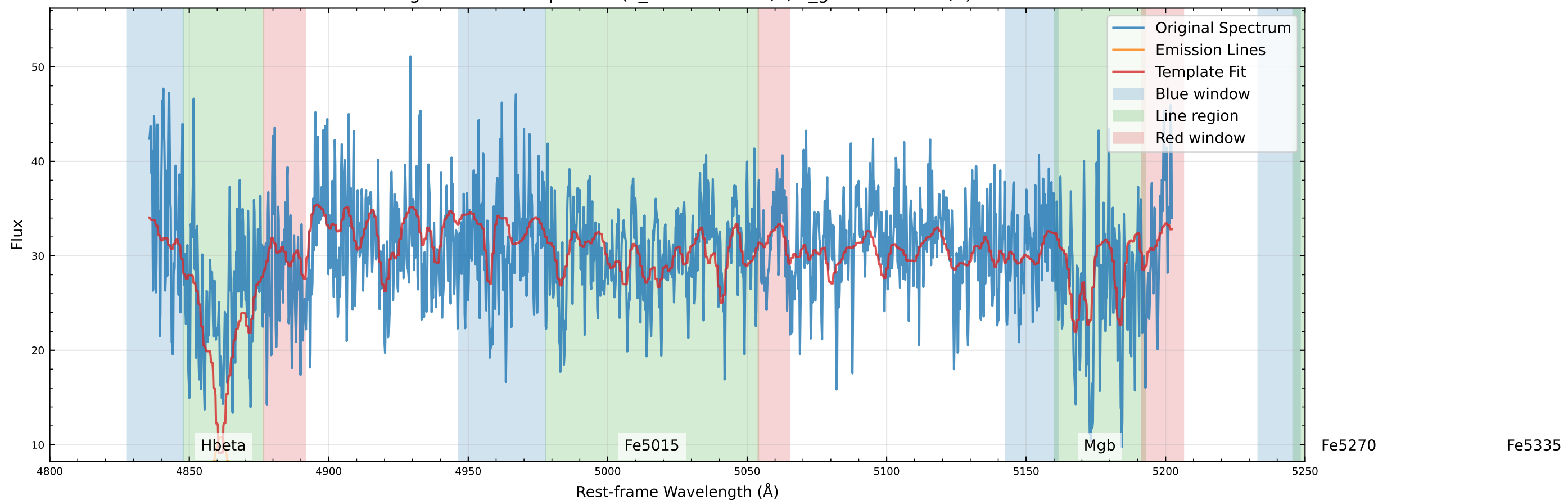
Original Data Comparison ( v_{\text{star}}=33.9 km/s, v_{\text{gas}}=106.4 km/s)
