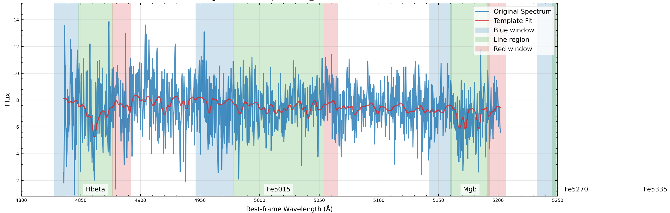
Original Data Comparison (v_star=-91.8 km/s)
