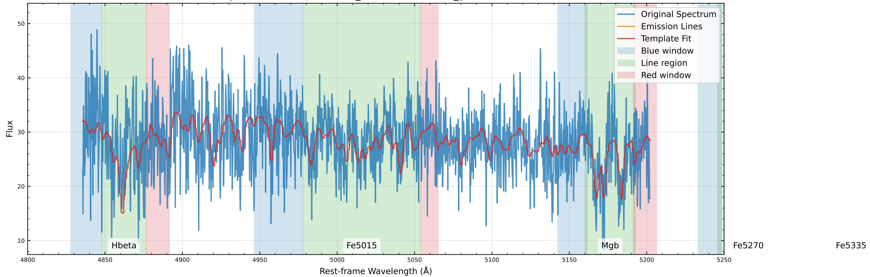
Original Data Comparison (v_star=-42.1 km/s, v_gas=94.1 km/s)
