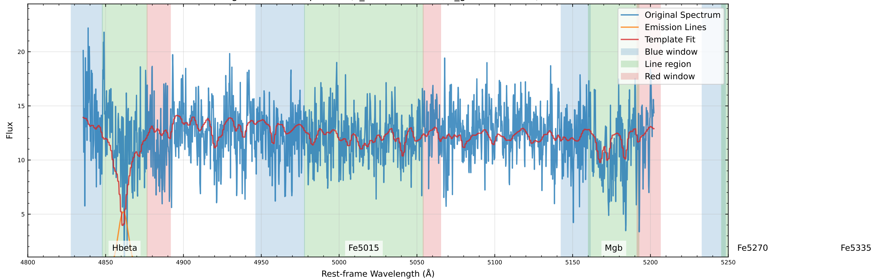
Original Data Comparison (v_star=32.9 km/s, v_gas=20.2 km/s)
