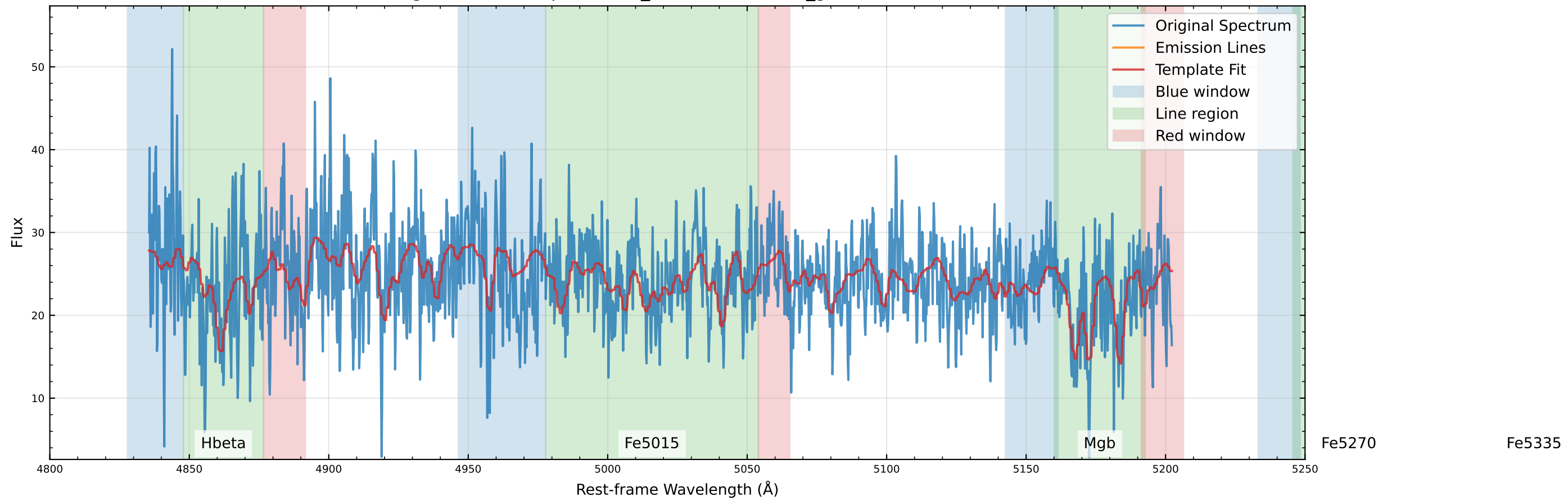
Original Data Comparison (v_star=-3.9 km/s, v_gas=138.7 km/s)
